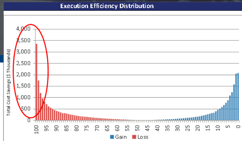
Sample high-grade bond manager trade distribution flags degrees that outliers drive costs
